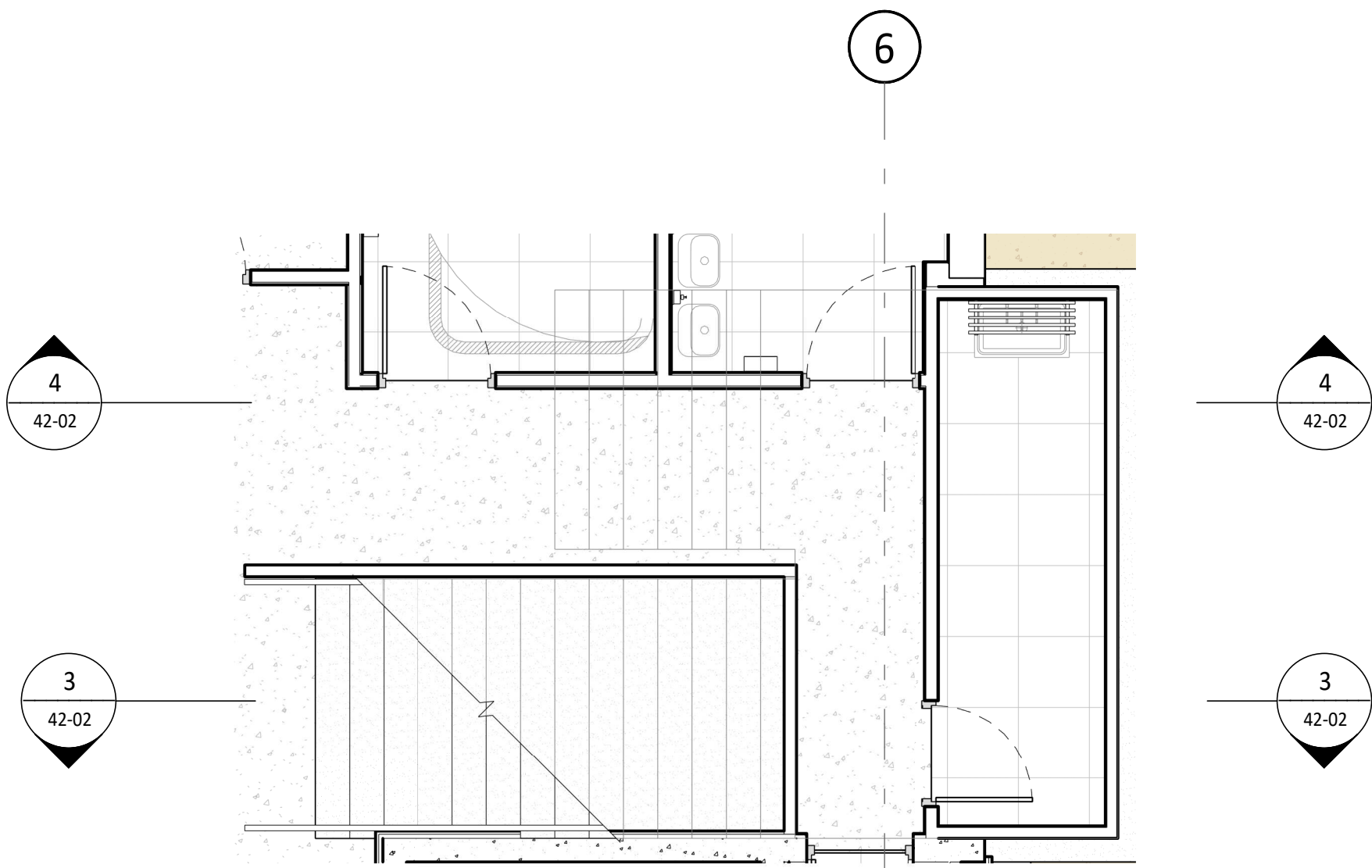
1 STAIR 02 - GROUND LEVEL 30-01 1 : 50
