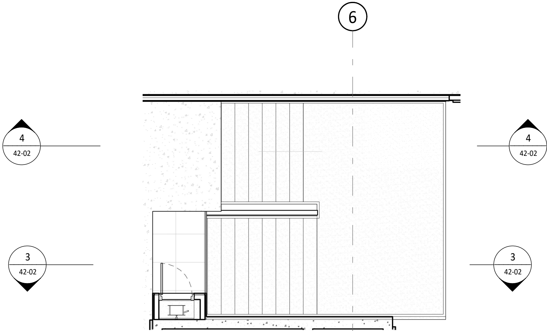
1 STAIR 02 - GROUND LEVEL 30-01 1 : 50
